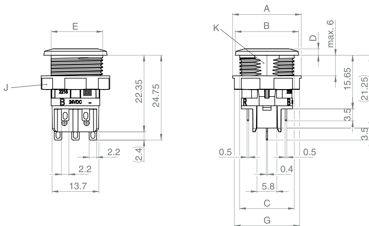
MSM II SPDT with Subminiature Microswitch and Solder Terminal
