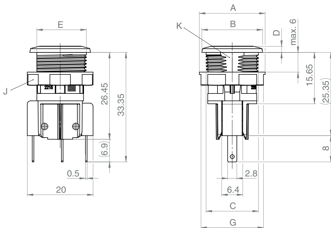
MSM II SPDT with Subminiature Microswitch and Solder Terminal
