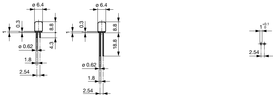
Drilling diagram
